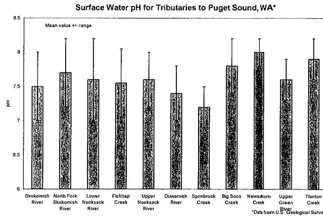
Figure 1. Surface water pH for Puget Sound tributaries (from U.S. Geological Survey)
